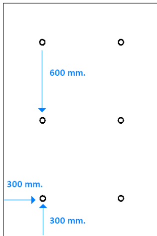
Plafondeiland 1200x1800
