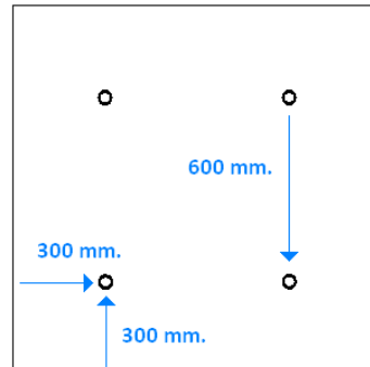
Plafondeiland 1200x1200
